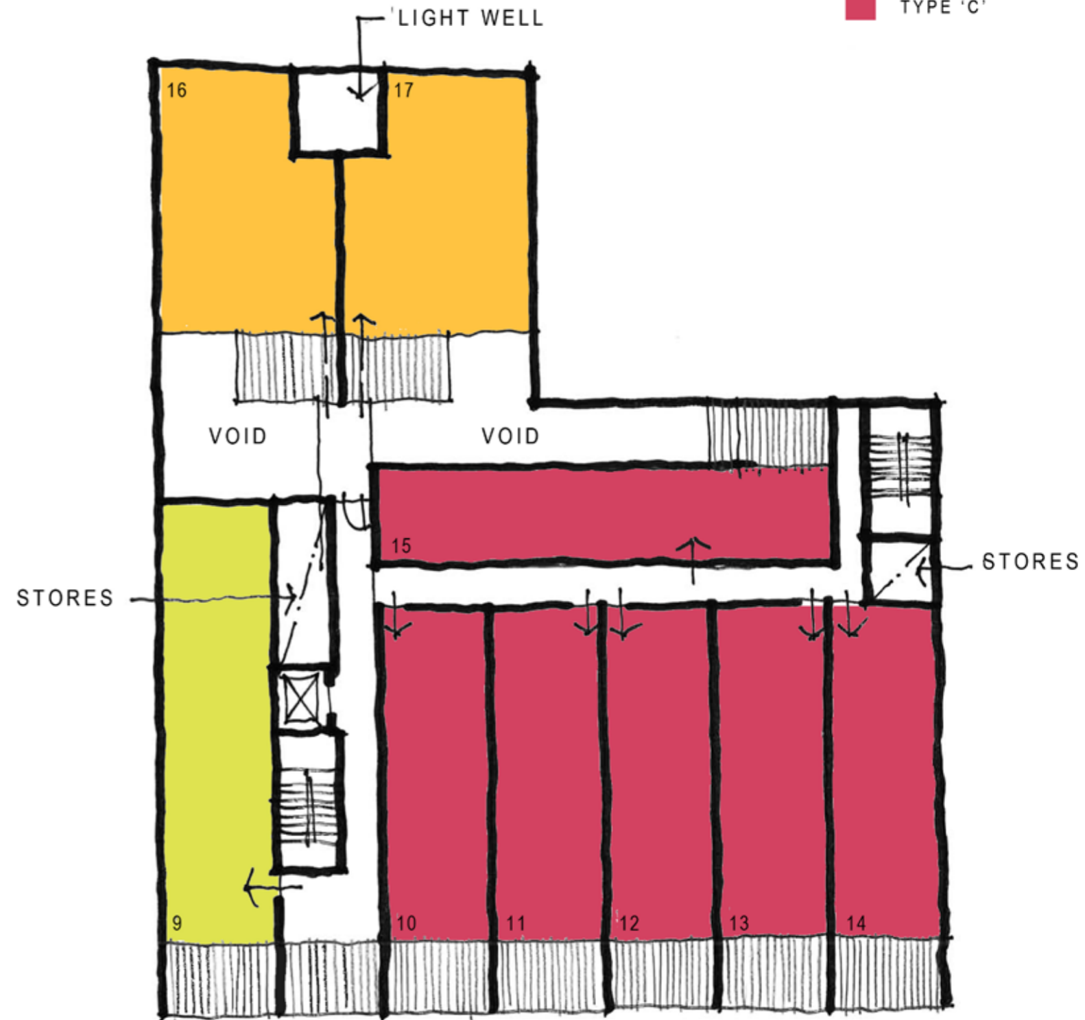
SECOND FLOOR PLAN 1:200 @ A3
