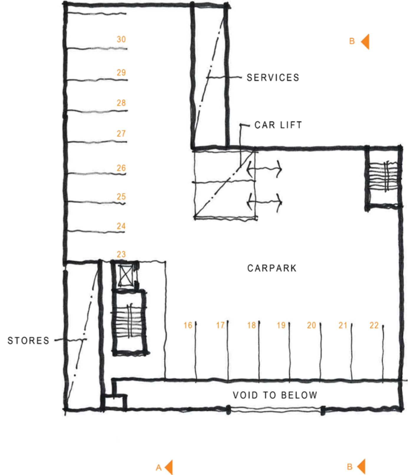
MEZZANINE PLAN 1:200 @ A3
