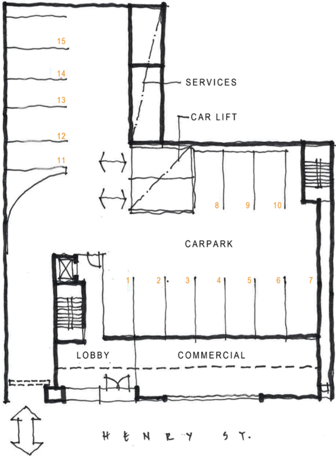
GROUND FLOOR PLAN 1:200 @ A3
